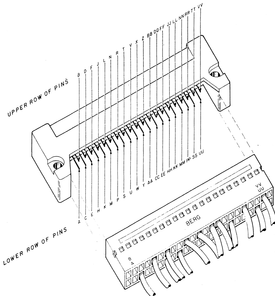
Figure 2-2 Berg Connector
